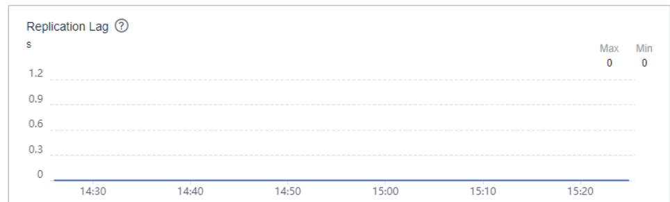
Figure 17-5 Replication Lag
